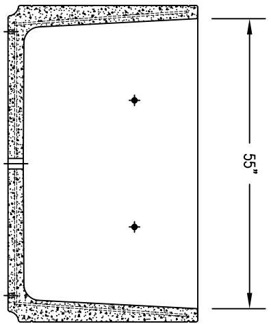
4 CROSS SECTION
