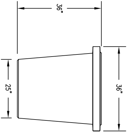
2 ELEVATION VIEW
