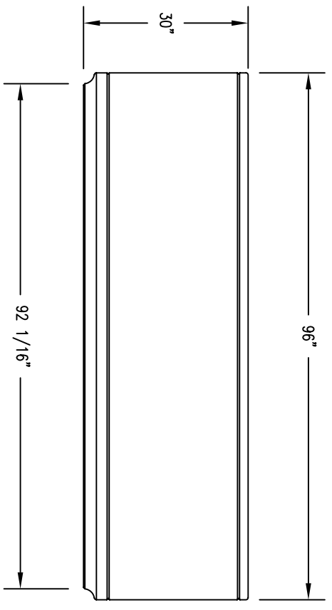
2 ELEVATION VIEW
