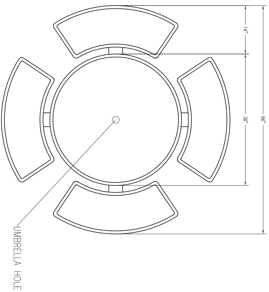
1 TOP VIEW SCALE 1/8"=1"
