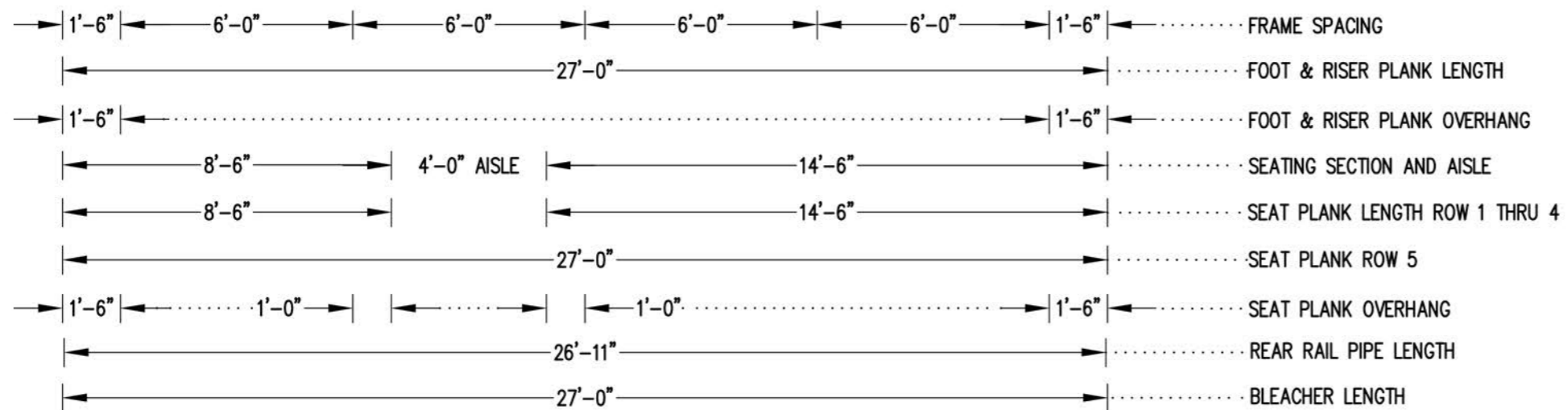
SEATING & FRAMING PLAN 1/4" = 1'-0" 74 NET SEAT @ 18" PER SEAT
