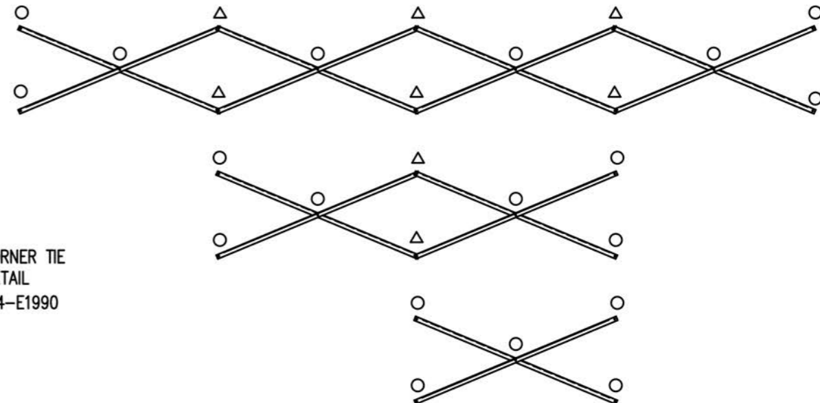
X-BRACE DETAIL N.T.S. ○ 7/16" X 1" GALV. MACH. BOLT △ 7/16" X 1.1/2" GALV. MACH. BOLT
