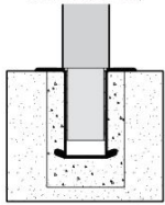
Inground Removable (Permanent Socket, Removable Post)
