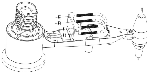
Figure 2: U-Bolt installation
