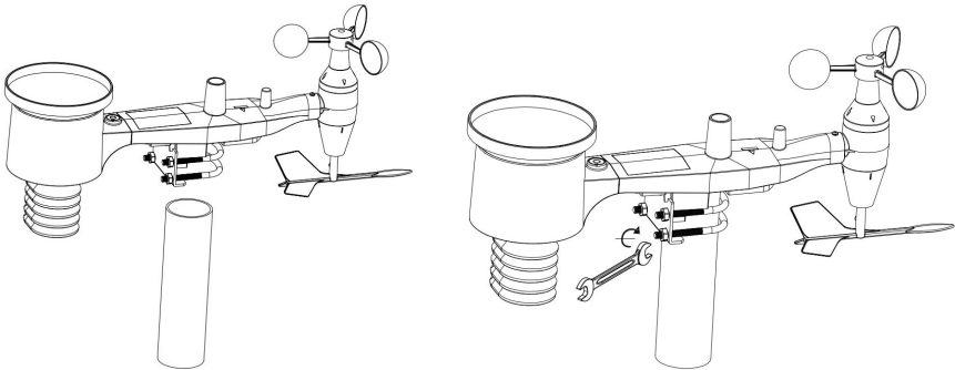
Figure 7: Sensor package mounting diagram
