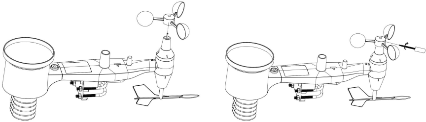
Figure 5: Wind speed cup installation diagram
