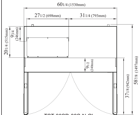
TST-60SD-08S-N-CL TOP VIEW
