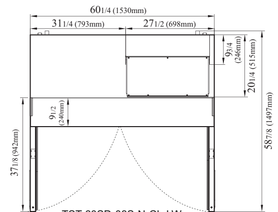
TST-60SD-08S-N-CL-LW TOP VIEW
