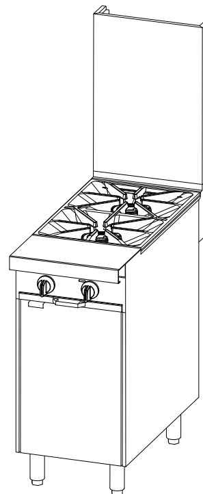
Model P18C-X with optional 24" flue riser and optional, removable cast iron grate top
