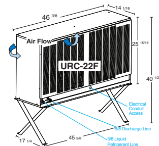
REMOTE AIR-COOLED
