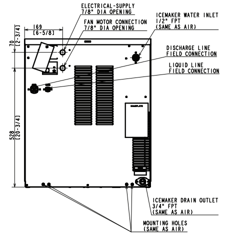
REMOTE AIR-COOLED
