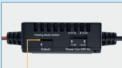
Fig: Parking Mode Switch
