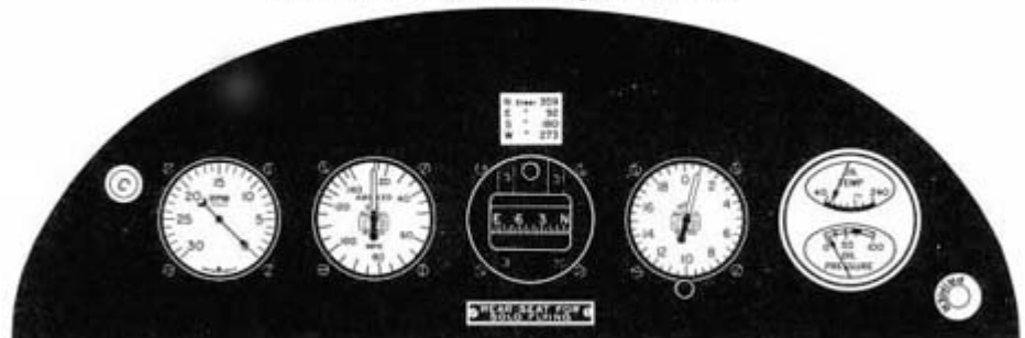
Cabin Heat Tachometer Airspeed Indicator Magnetic Compass Non-Sensitive Altimeter Engine Oil Gauge Engine Primer
