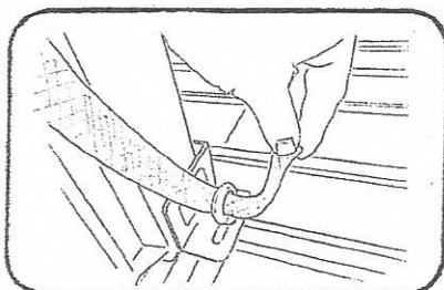
Thread ratchet strap through eye nuts strap must go diagonally across the box In order to secure in place.
