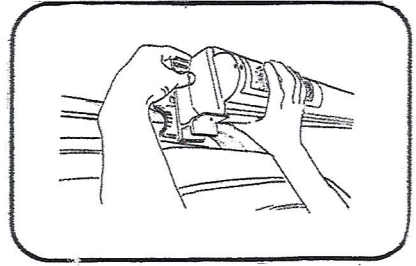
Slide awning into awning kit open casing . Drill a 4mm hole and secure with bolts provided as per awning instructions
