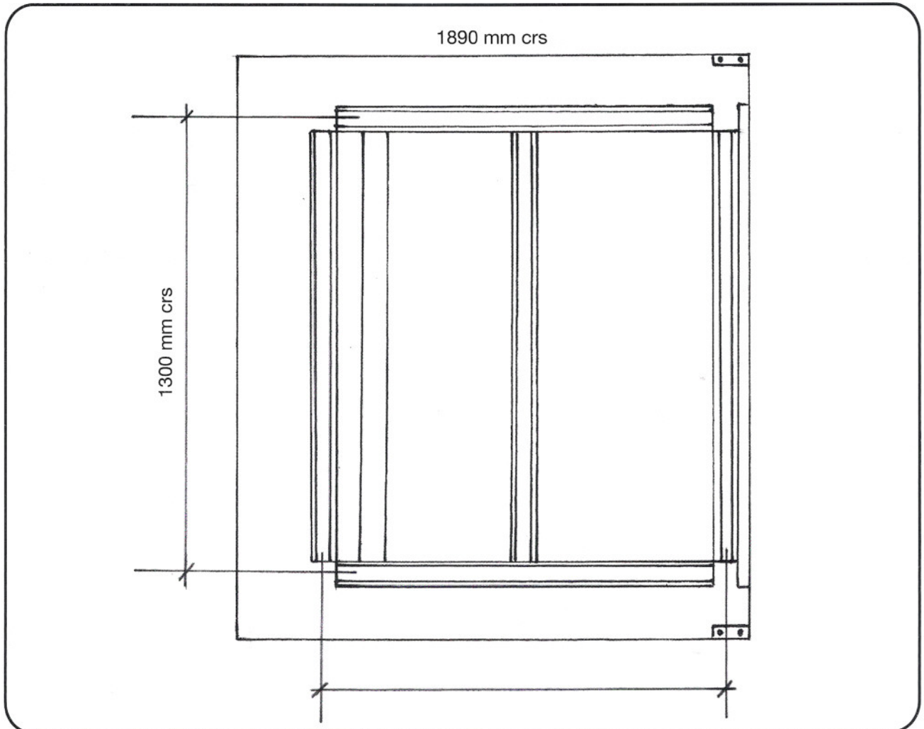
Plan View Rooftent base rail centres
