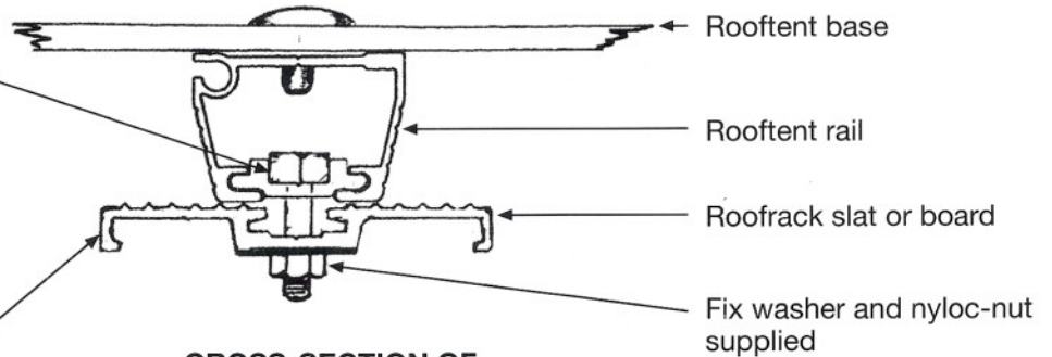
CROSS-SECTION OF INSTALLATION ROOFTENT TO ROOFRACK
