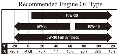
Engine Oil Temperature Recommendations
