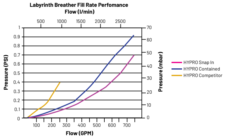
As depicted in the graph above, the Hypro Labyrinth Breather consistently performs at a higher fill rate and lower pressure than the typical competitor.
