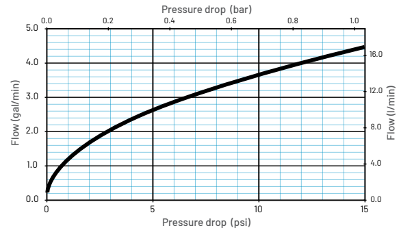
PROFLO NOZZLE BODY PERFORMANCE CURVE
