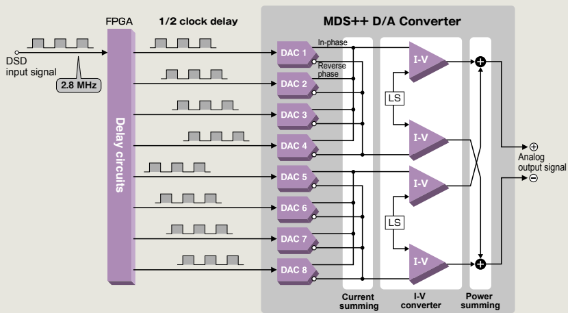
MDSD principle block diagram
