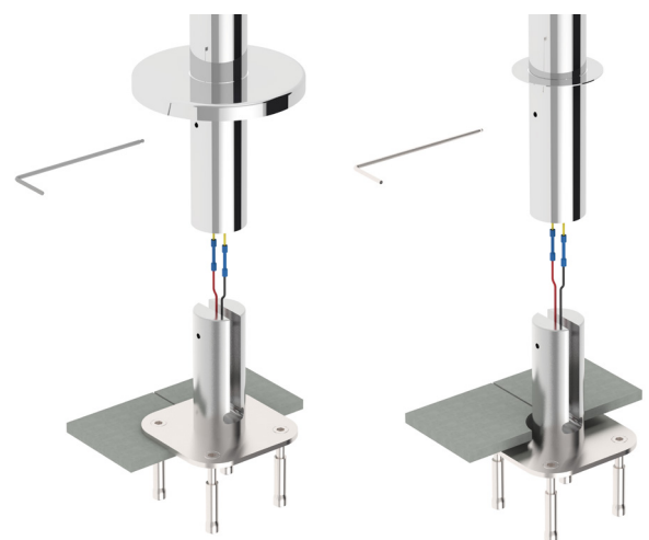
Over Tile Installation
