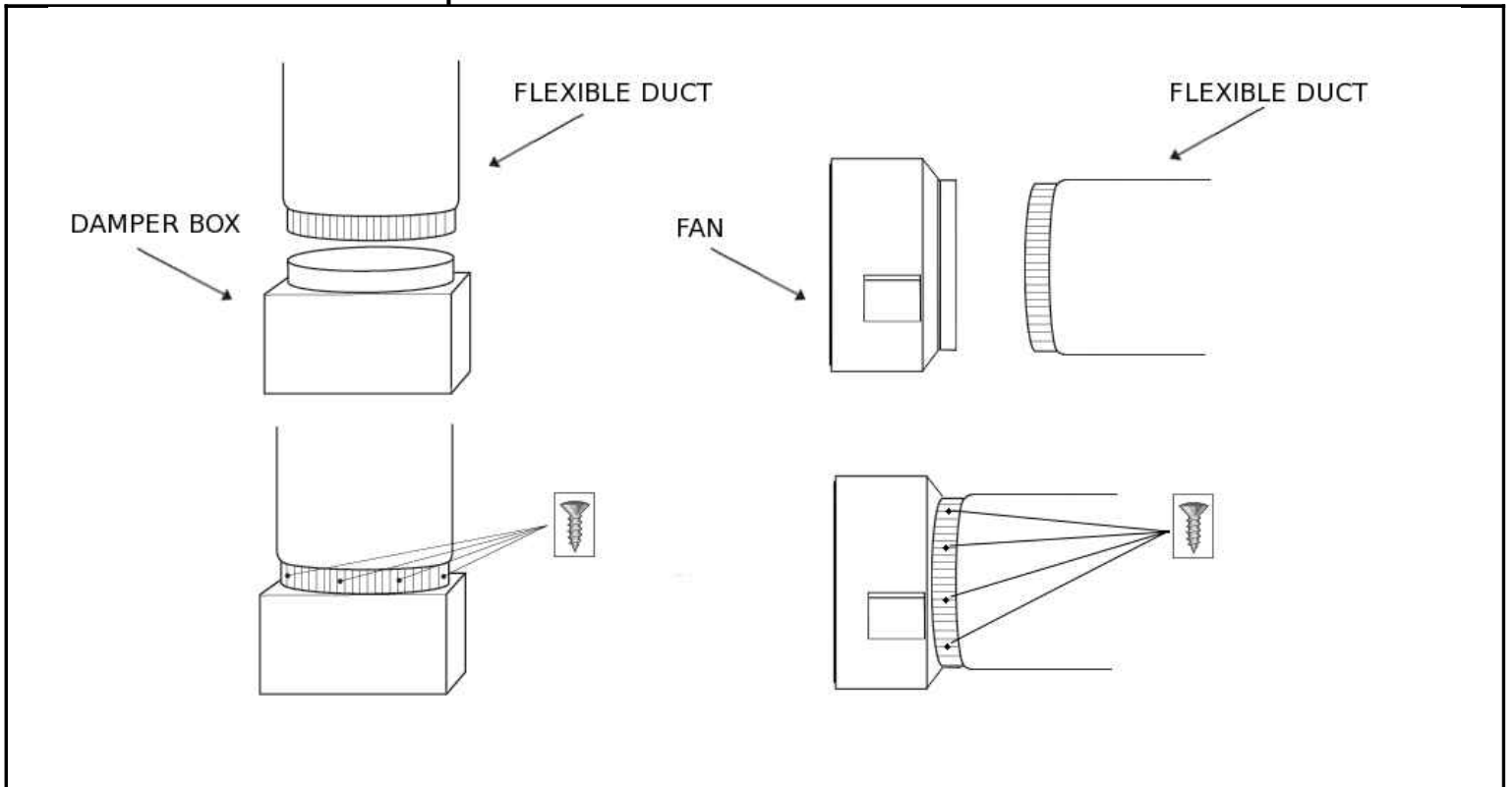
FIGURE 5 – Duct to Damper and Duct to Fan Connections
