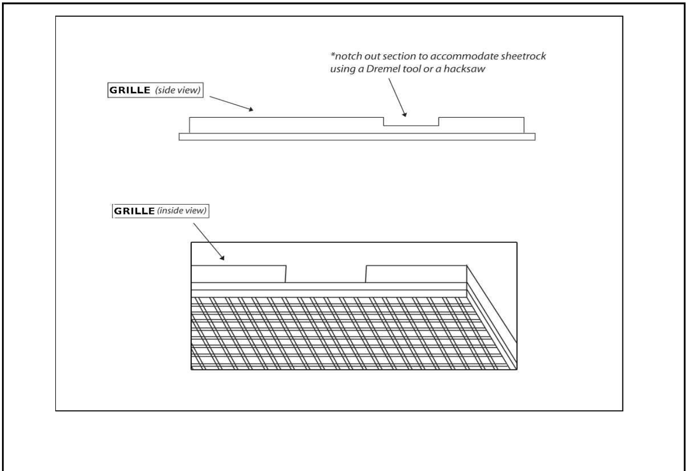
FIGURE 4 – Grille Notch -- ONLY 16" O/C Installations.
