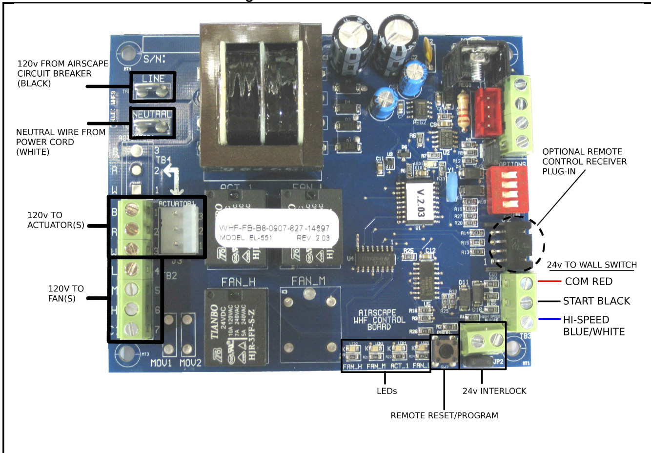
FIGURE 11 – Control Board Diagram
