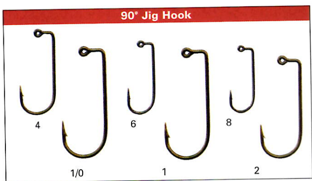
4660 (Bronze) 4663 (Red) Round bend, standard wire, 90° bend, flat eye Uses: Jigs, Flies for float fishing
