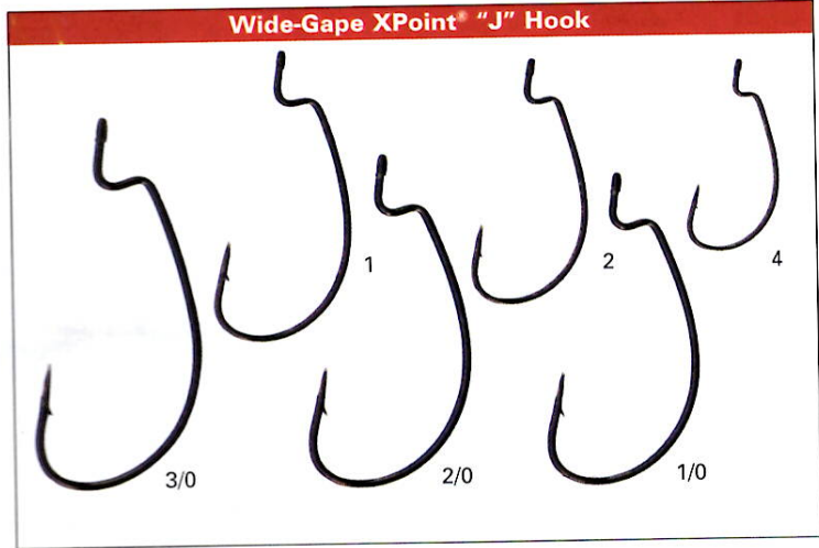
X-15 (Black Nickel) Wide-gape sproat bend, straight-eye standard wire, XPoint Uses: Bass, Pike & Saltwater Flies, Keeled Flies & use with Vinyl Bass Baits
