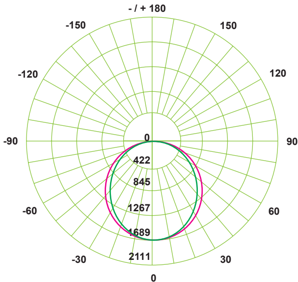
Polar Curve
