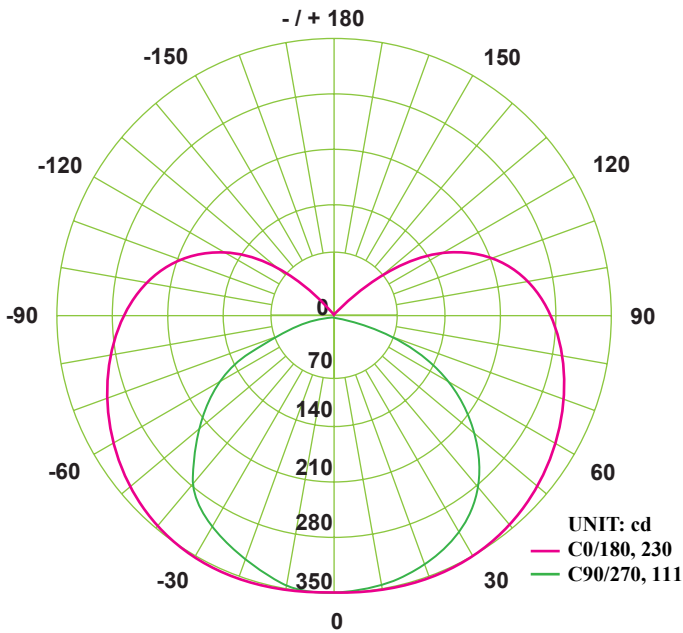
Polar Curve
