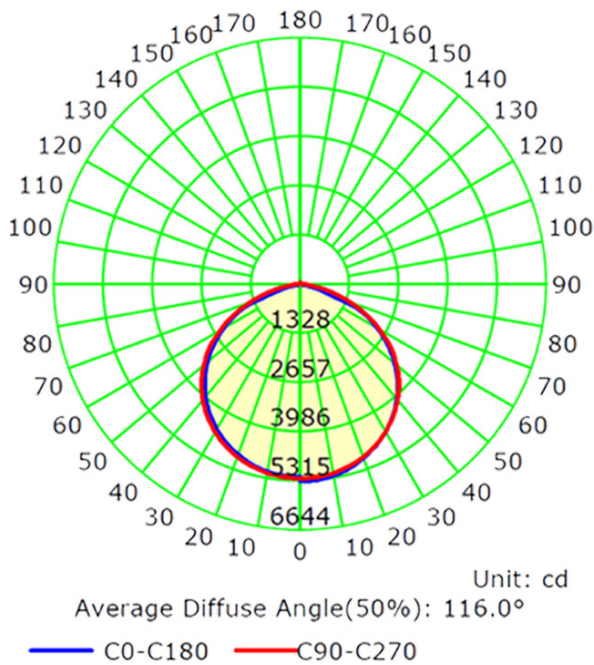
Polar Curve
