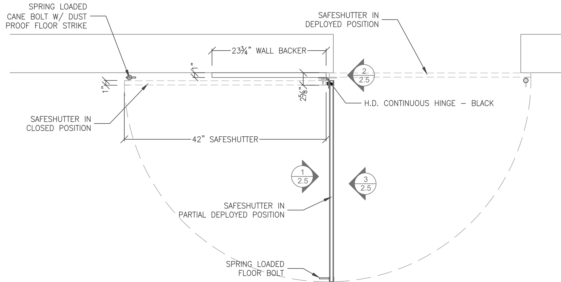
1 UL3 SAFESHUTTER 2.4 SS-WB-3660-WHWHI-UL03 SCALE: 1" = 1'-0"
