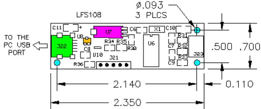
Figure 8 - General Dimensions, LFS108B
