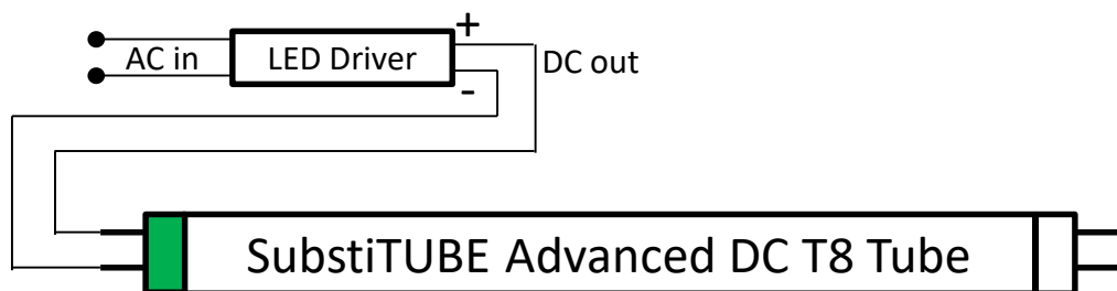
SubstiTUBE® Advanced DC T8 Tube Wiring
