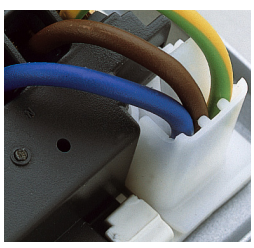
A simple but effective cord grip securely holds the cable in connection units
