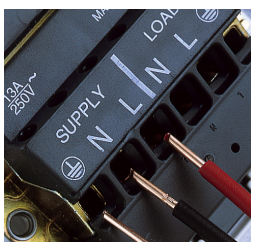
In-line terminals means that cables can be cut to the same length. White printing gives instant terminal identification
