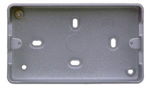
K8902 ALM 4 x 20mm & 4 x 25mm Knockouts 46mm Deep Box
