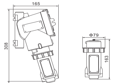
Plug
