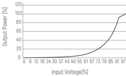
Dimming Curve
