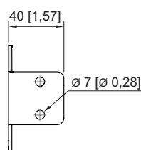
Mounting bracket for surfaces
