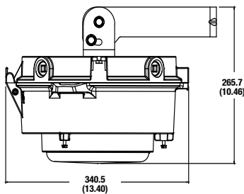
Trunnion Mount
