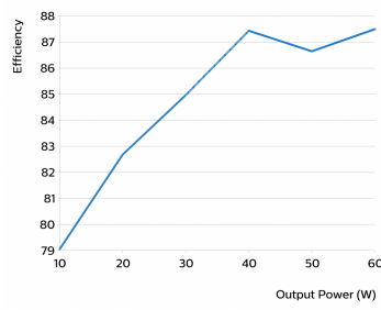
Efficiency versus output power
