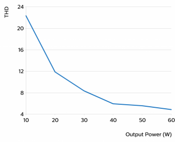
THD versus output power
