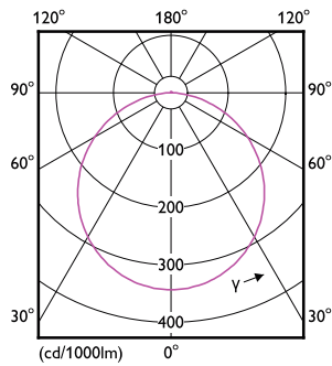
Downlight DN020 G3 WW 18W D175 SNI
