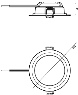
DN020B G3 LED4/WW 4.5W 220-240V D90 SNI
