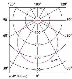
Downlight DN020 G3 WW 4,5W D90 SNI
