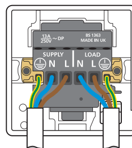
Supply and non flexible load cables
