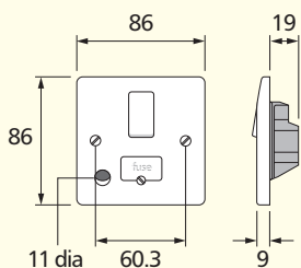
Products with front flex outlet
