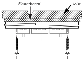
Figure 2 - Mounting Ceiling Rose base
