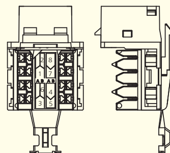
RJ45 Cat.6 Screened K5746S - LU6C, K5846S - Euro
