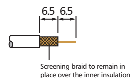
TV Co-axial cable stripping details
