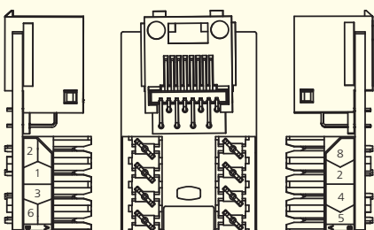
RJ45 Cat.5e LU6C K5745
