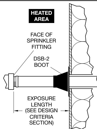
FIGURE 5 SPRINKLER BARREL EXPOSURE LENGTH
