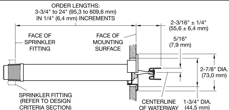
FIGURE 3 SERIES LFII DRY TYPE RESIDENTIAL HORIZONTAL SIDEWALL SPRINKLERS WITH STYLE 20 RECESSED ESCUTCHEON
