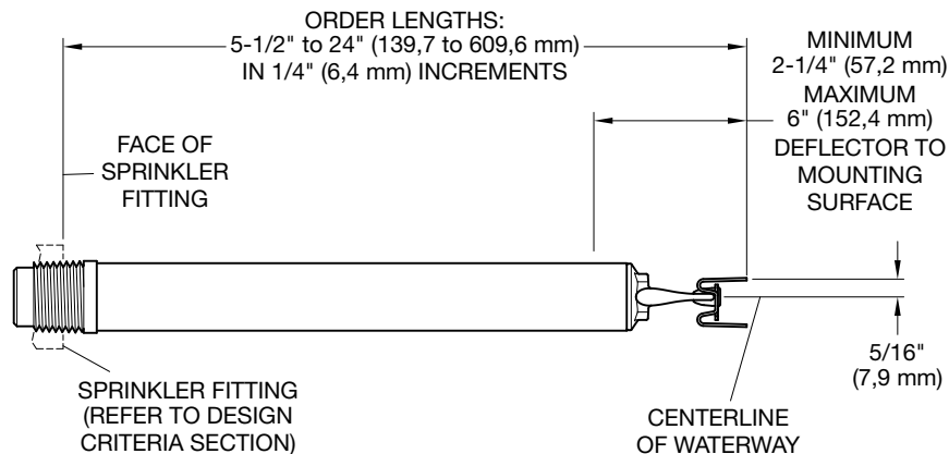
FIGURE 2 SERIES LFII DRY TYPE RESIDENTIAL HORIZONTAL SIDEWALL SPRINKLERS WITHOUT ESCUTCHEON
