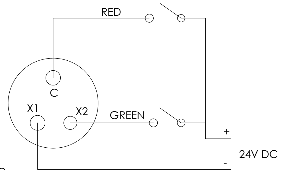
PNP WIRING FOR 24V DC VERSION
