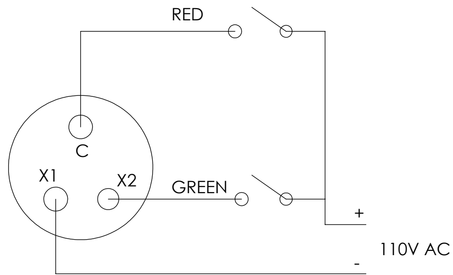
PNP WIRING FOR 110V AC VERSION
