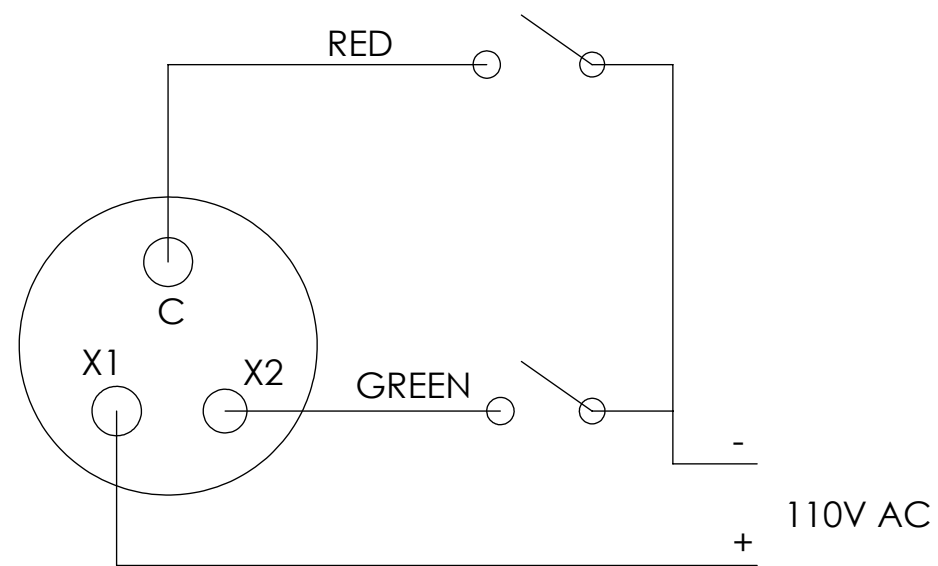
NPN WIRING FOR 110V AC VERSION
