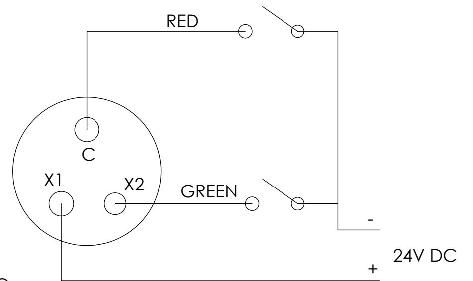
NPN WIRING FOR 24V DC VERSION
