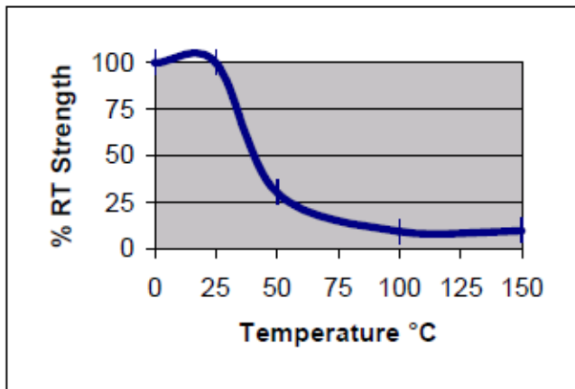
Tested at temperature.
