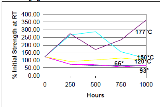
Cured for 5 days at 22°C on steel with no induced gap, aged at temperature indicated and tested at 22°C.
