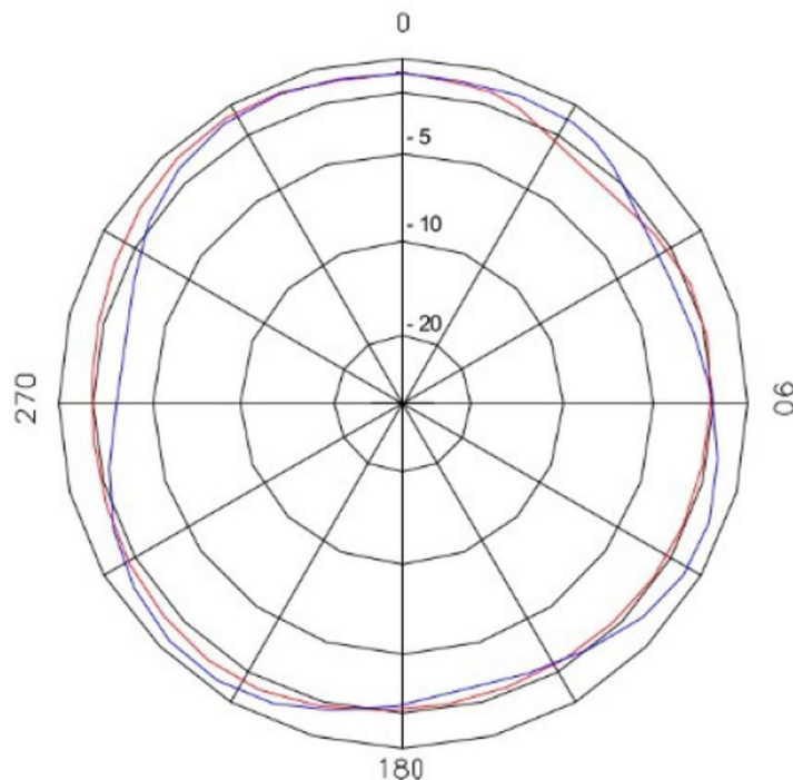
Horizontal Pattern
