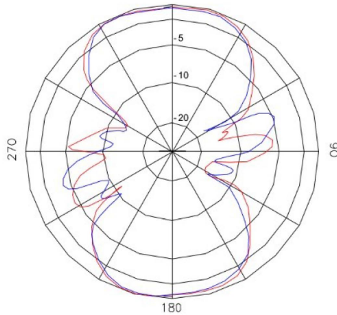
Vertical Pattern
