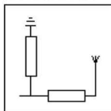
Typical config.1
