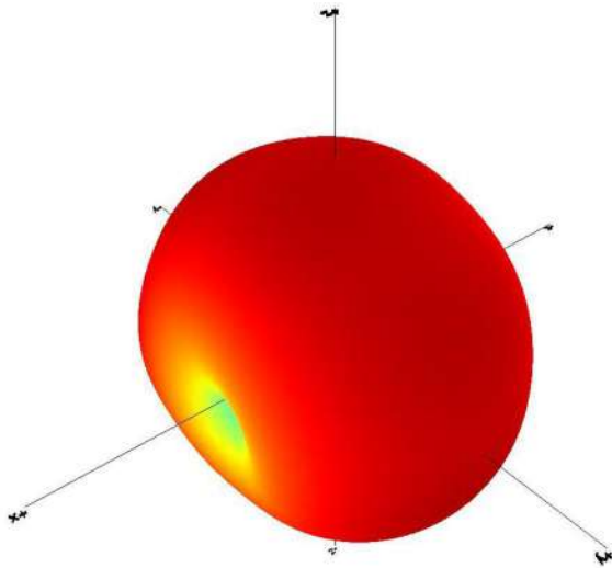
824MHz
