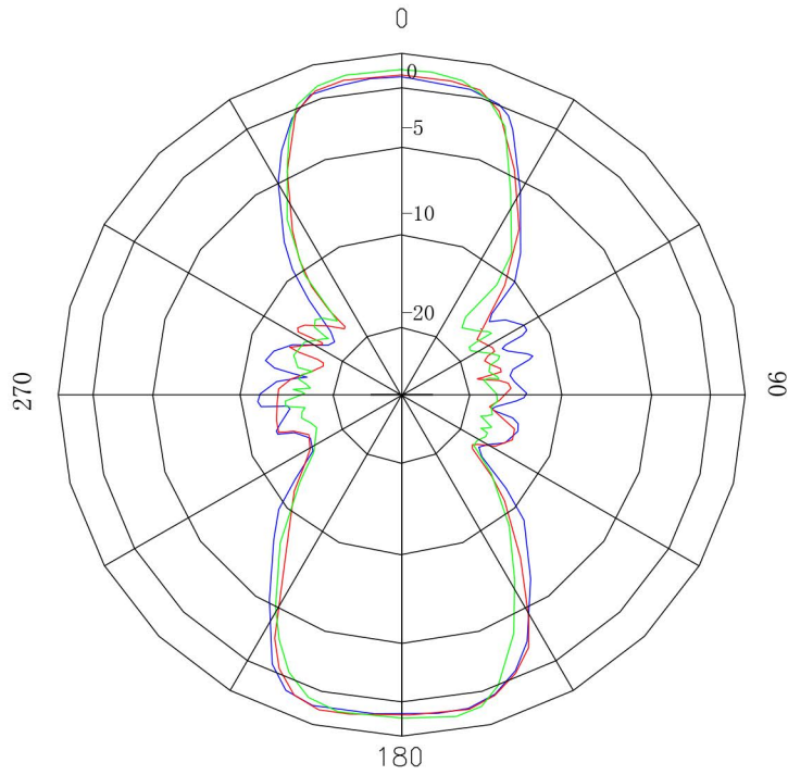
Vertical Pattern
