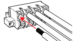
Image C - Tow-Pro Classic Connector (Green) Image C - Connecteur Tow-Pro Classic (vert) Image C - Conector de Tow-Pro Classic (Verde)
