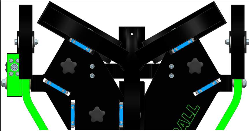
Figure 5: Typical motor / wheel positioning for real baseballs - motors are located at center position
