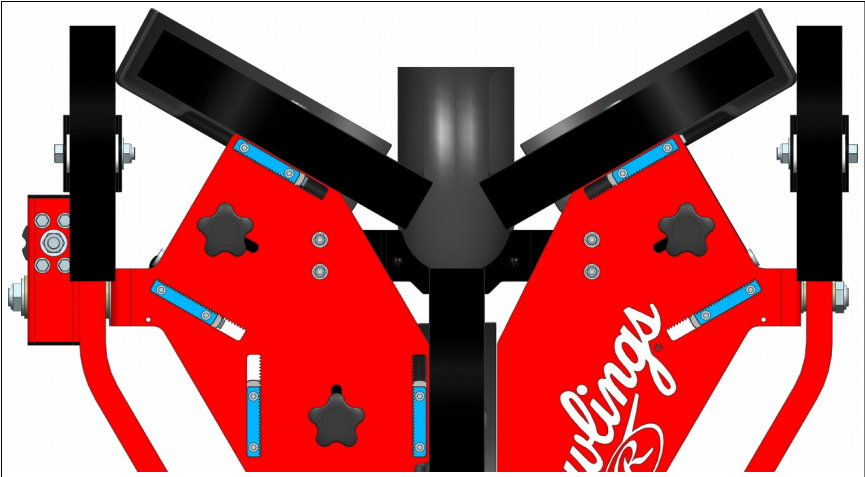
Figure 4: Typical motor / wheel positioning for real softballs - motors are located at outermost position
