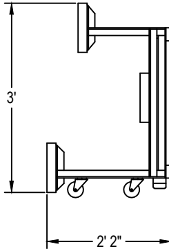
STORAGE POSITION
