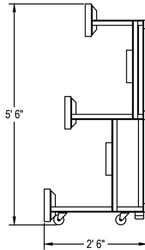
STORAGE POSITION
